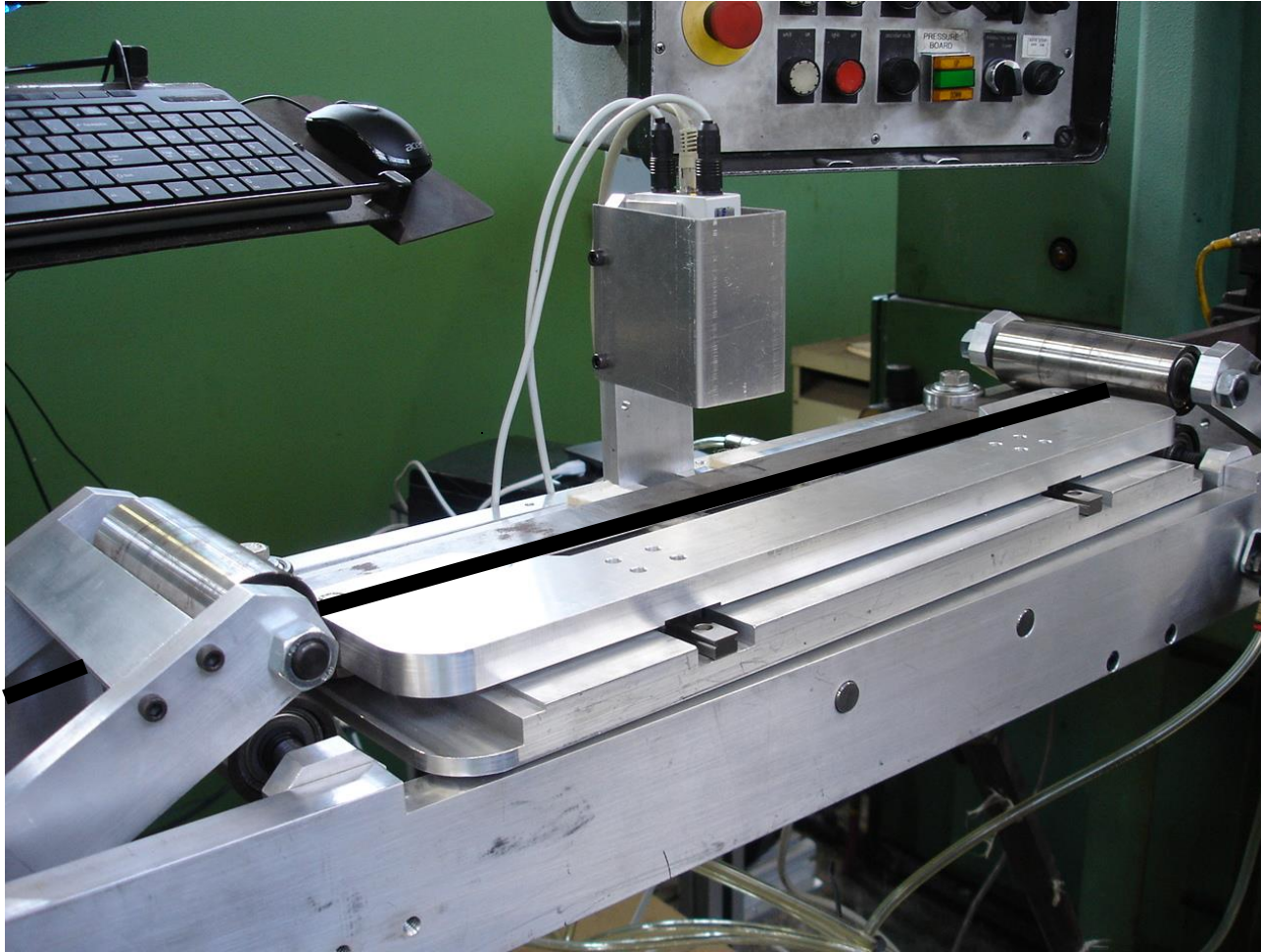
Strip Material Continuous Camber Gauging System Noncontact Through Beam Laser Sensor
